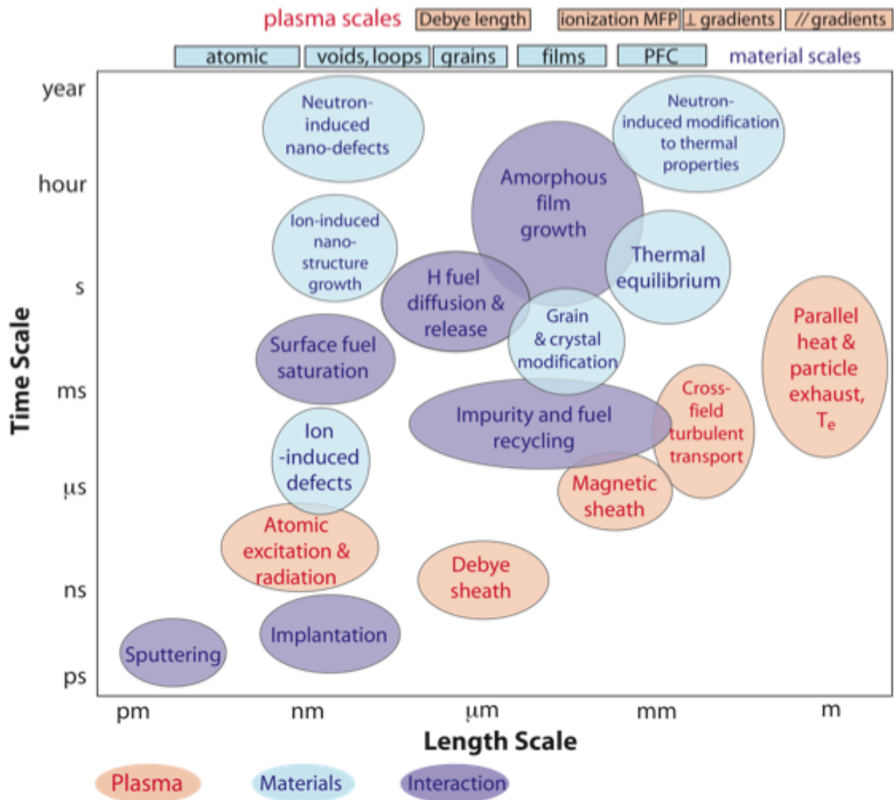
Figure 2.2.1. Overview of the coupled multi-scale phenomenon associated with plasma-materials interactions.
