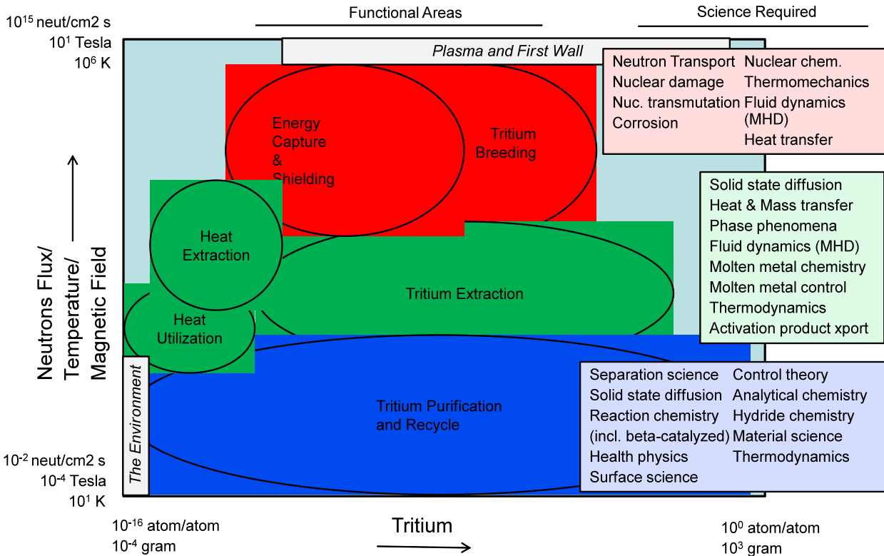
Figure 2.4.1: Science associated with the Harnessing Fusion Power functions plotted against the vast range of tritium, neutron, temperature and magnetic field parameter space extending between a fusion plasma and the environment
