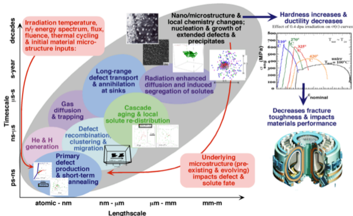
Figure 2.3.1. Radiation-induced microstructural evolution is a multi-scale phenomenon spanning enormous spatial and temporal regimes.
