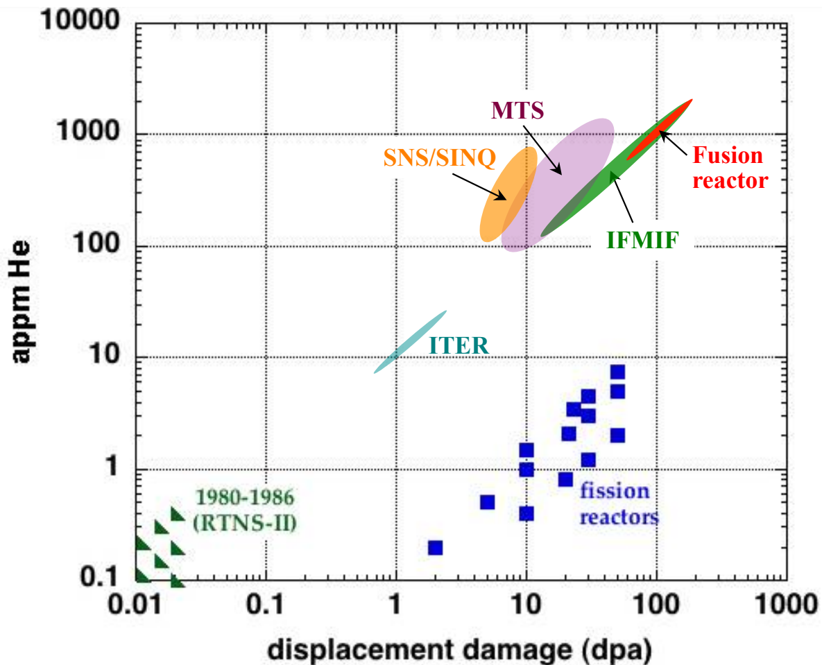
Figure 3.3.1. Summary of helium generation and displacement damage levels in ferritic steels for various neutron irradiation sources for ~2-4 year exposure times.
