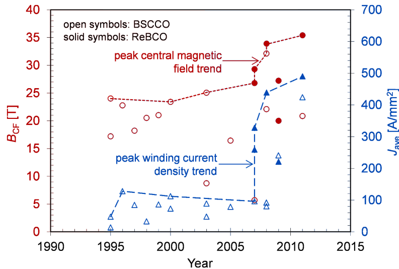
Figure 3.3.2. Highest fields and overall winding current densities generated by HTS R&D magnets during the last 16 years. The two conductors featured here, REBCO and round wire Bi-2212, complement each other, one being more suitable for certain applications than the other. The ideal HTS conductor would in fact have the round wire attributes of Bi-2212 and the high flux pinning capability and high irreversibility field of REBCO, properties which would allow the very high current cables needed for DEMO or other large fusion machines [3.24].
