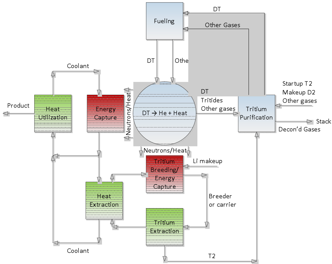
Figure 3.4.1: Key Harnessing Fusion Power functions including (red) tritium breeding and neutron energy capture in the blanket, (green) extraction of fusion energy and bred tritium, (blue) purification and recycle plasma exhaust
